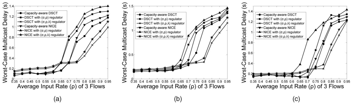
Fig. 6. The worst-case delay performances when each of the three groups is fed with the same (a) 64-Kbps audio streams, (b) 1.5-Mbps video streams, and (c) one 1.5-Mbps video stream and two 64-Kbps audio streams.
