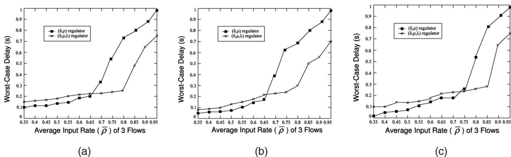
Fig. 4. The worst-case delay performances when there are (a) three 64-Kbps audio streams, (b) three 1.5-Mbps video streams, and (c) one 1.5-Mbps video stream and two 64-Kbps audio streams in the network.
