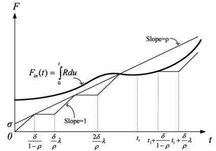
Fig. 2. An example of the operations of a (\sigma, \rho, \lambda) regulator. The x -axis represents the communication time, and the y -axis represents the amount of data from the stream since the beginning of the communication. R is the traffic instantaneous input rate and \lambda = \frac{1}{(1-\rho)} is the traffic control factor of the (\sigma, \rho, \lambda) regulator.
